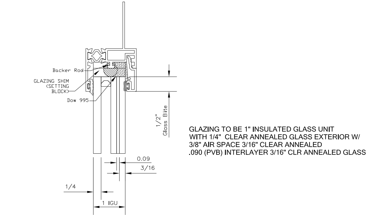
I. FIXED WINDOW GLAZING DETAILS
