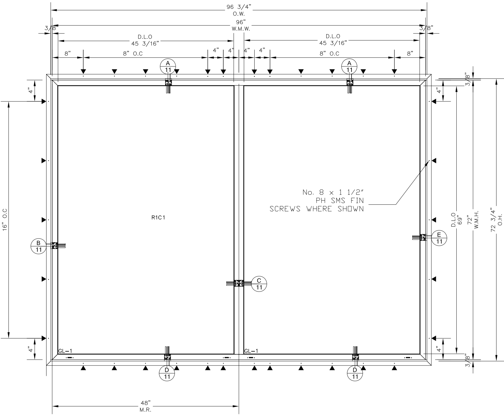
SPECIMEN 2A G845 QTY. 4 THUS Hurricane Glazed
