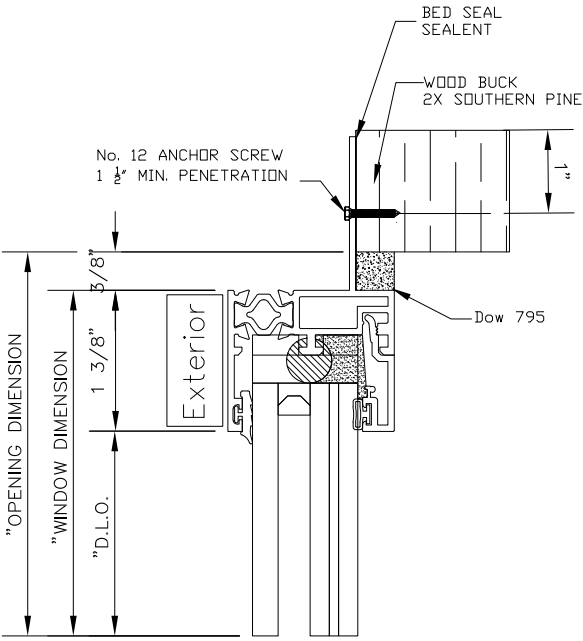
A HEAD Frame Depth: 1.625
