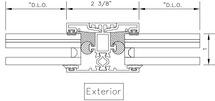
C MEETING RAIL Frame Depth: 1.625
