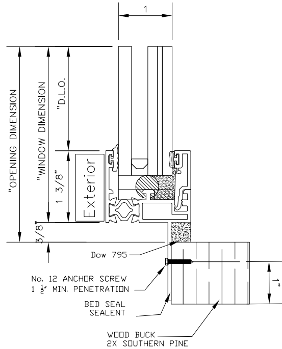
D SILL Frame Depth: 1.625
